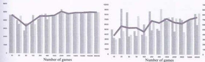
Figure 3. The score reached as games progressed for three different trials. In read the average value. On the left a random policy is adopted to learn Q(.), on the right an e-greedy policy has been implemented.
