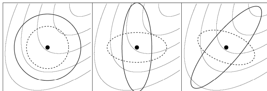
\mathcal{N}(0, \sigma^2 \mathbf{I})
